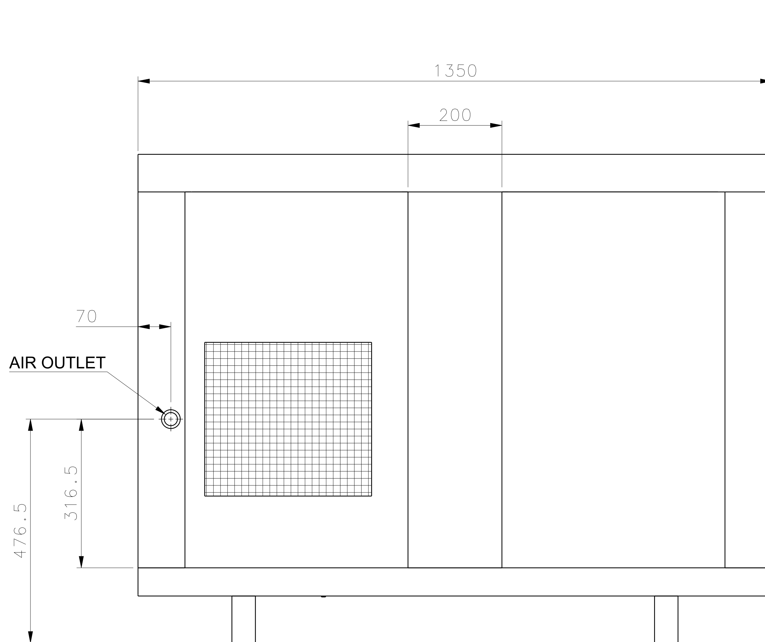
Rear view Scale: 1:5
