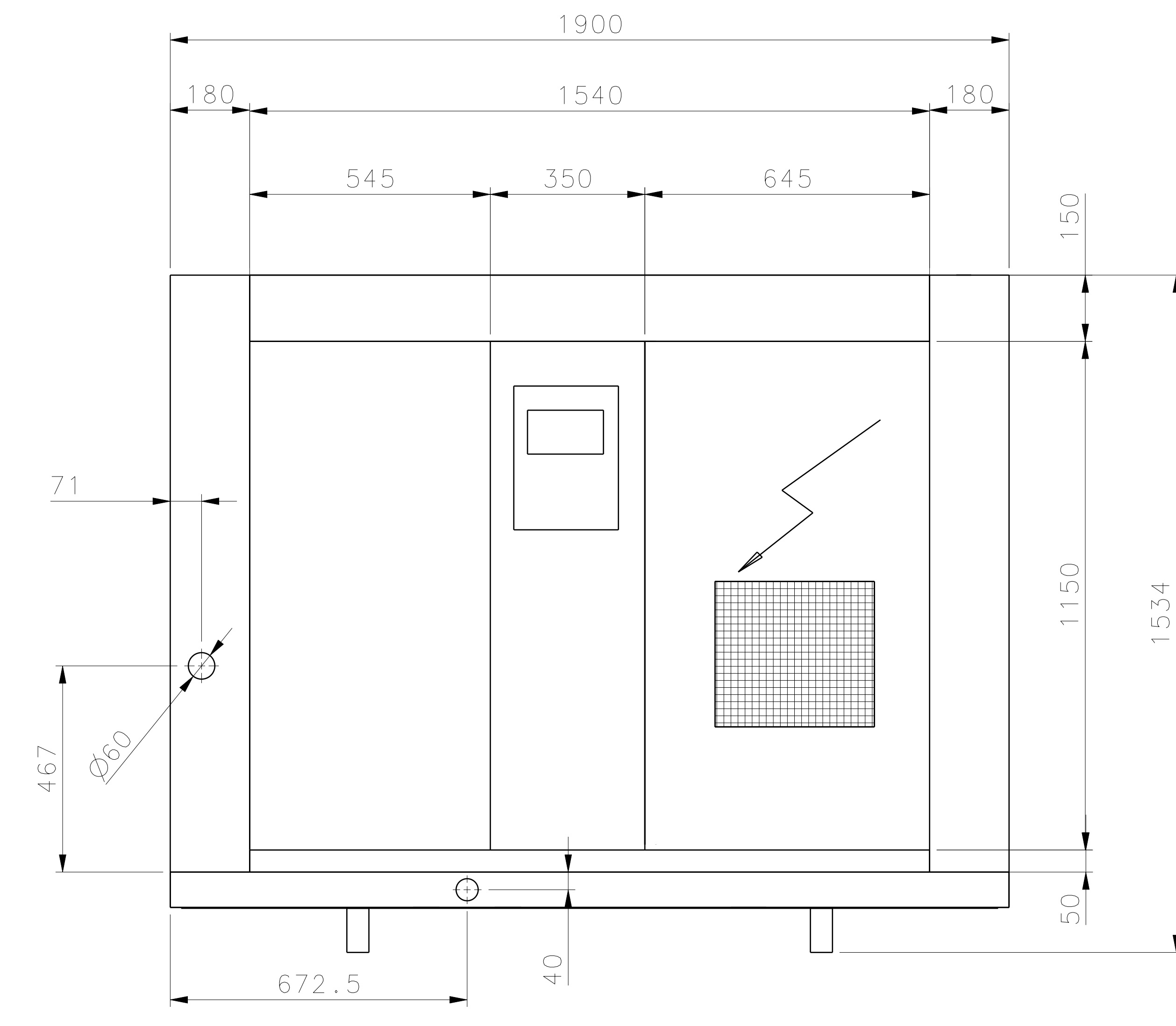
Front view Scale: 1:8
