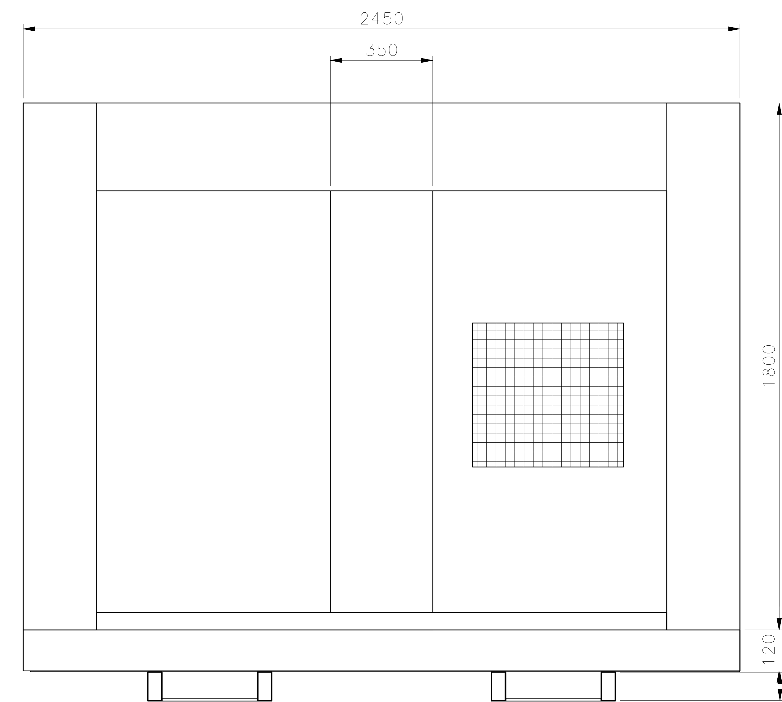
Rear view Scale: 1:8
