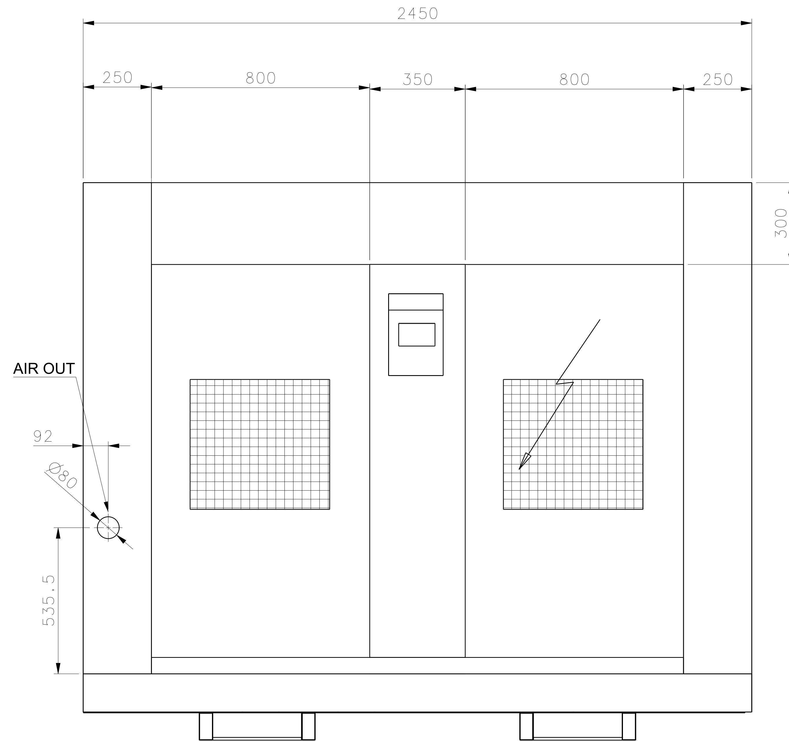
Front view Scale: 1:8
